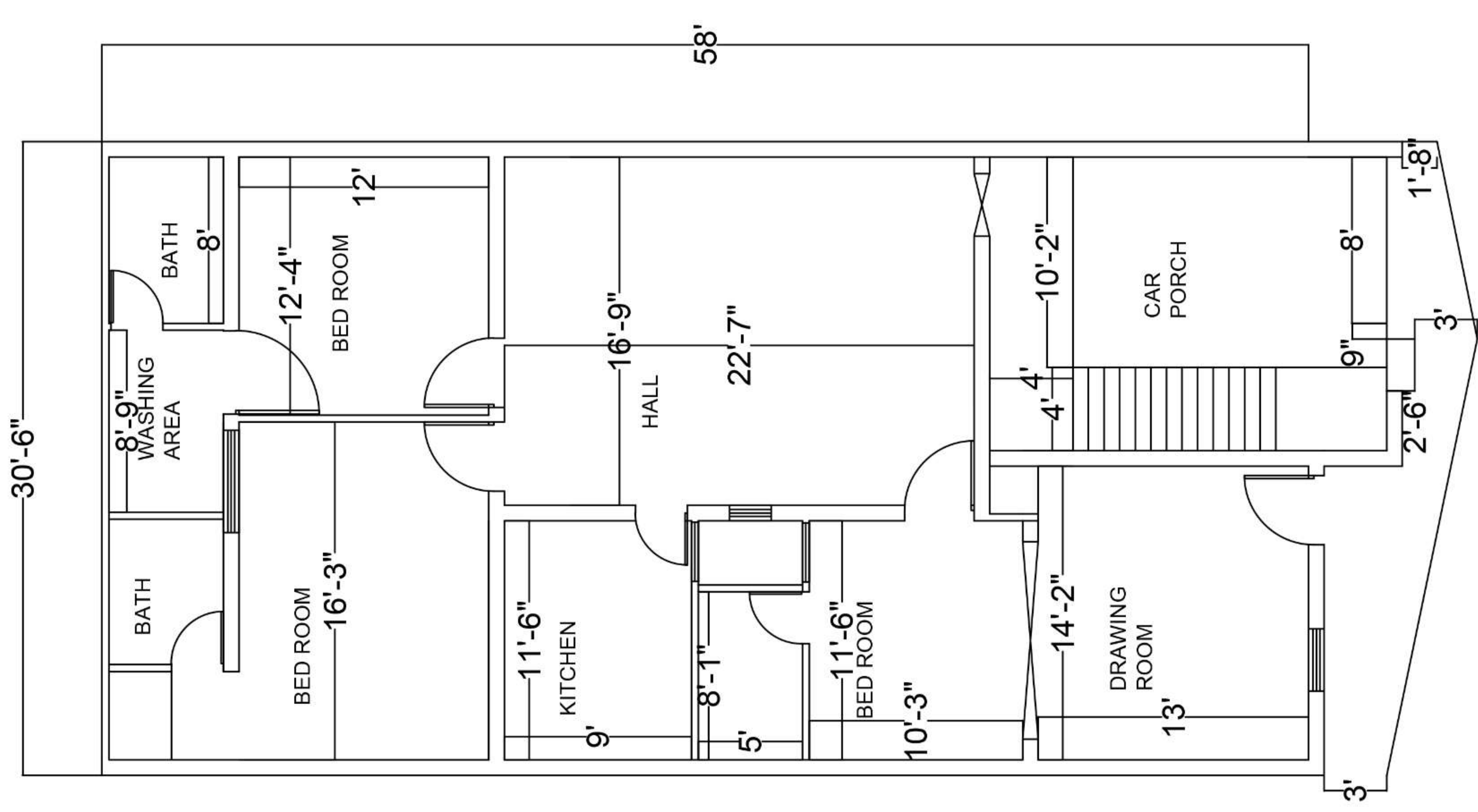
Blue Print
